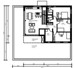
0. Stock
